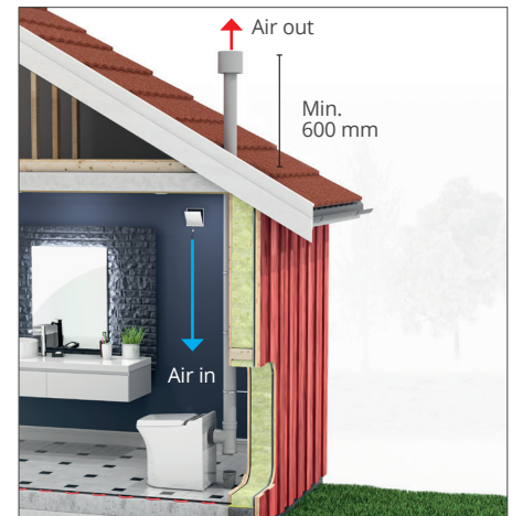
Air inlet high in wall, internal mounted flue (maximum length 5,5 m)
