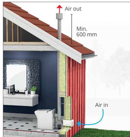
Air inlet behind toilet, internal mounted flue (maximum length 5,5 m)
