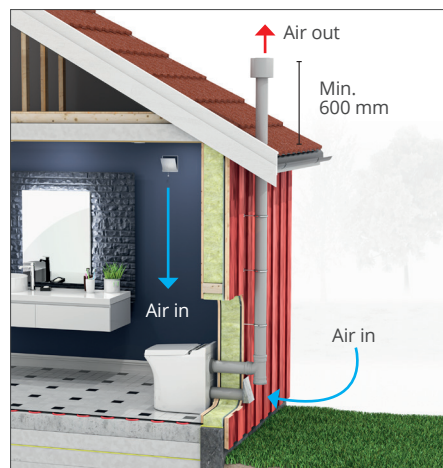
Additional air-intake, extractor fan in same room, external mounted flue (maximum length 5,5 m)
