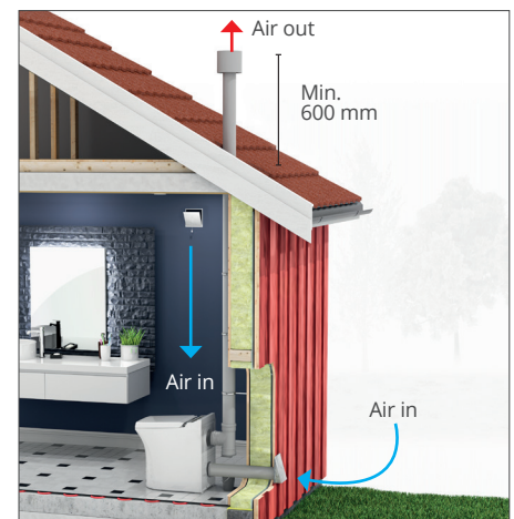
Additional air-intake, extractor fan in same room, internal mounted flue (maximum length 5,5 m)
